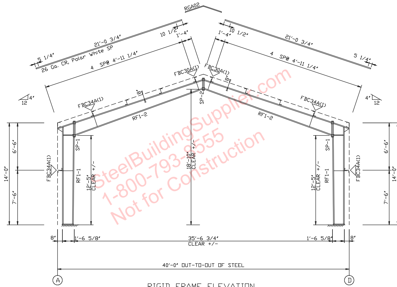
RIGID FRAME ELEVATION FOR FRAME LINE 2
